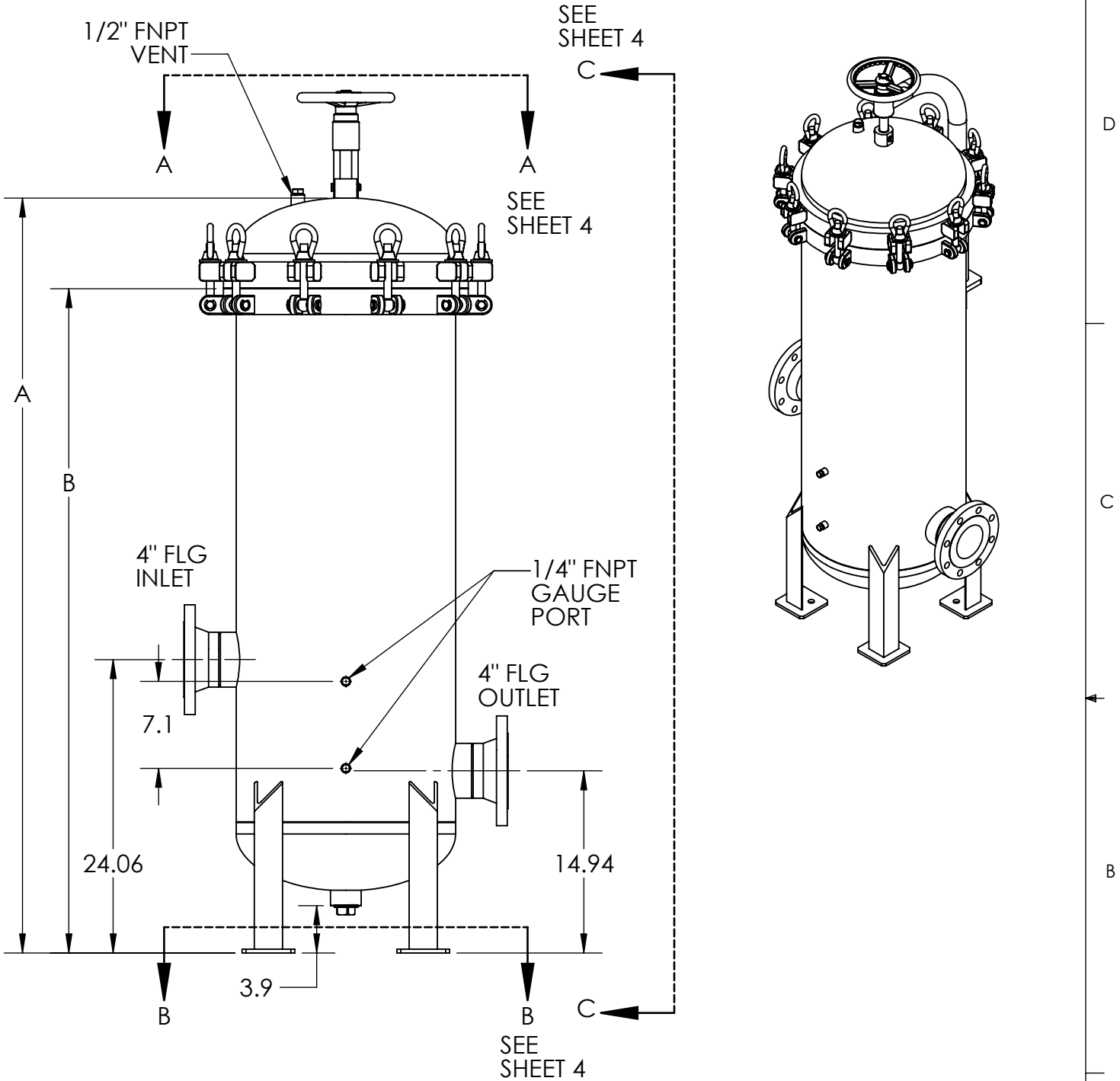
REFERENCE ENGINEERING DRAWING 21133
