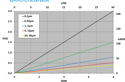
10" Filterkerze, in Wasser, 21°C
